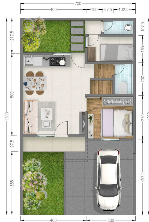
Denah Lantai Dasar
